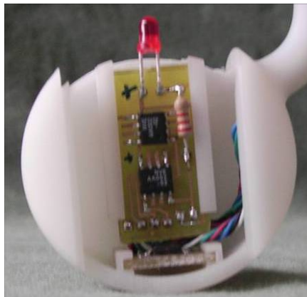
Fig. 6. Detail of the circuit boards mounted in the support developed for the sensors used
