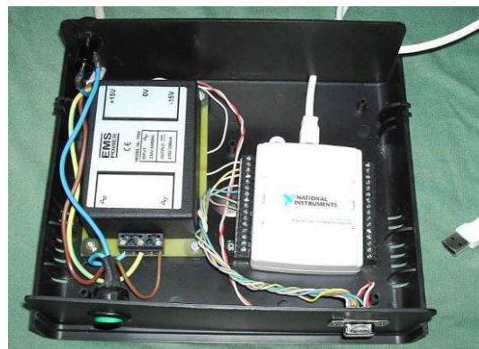
Fig. 8. Acquisition box with the DAQ and the power source used in our acquisition system
