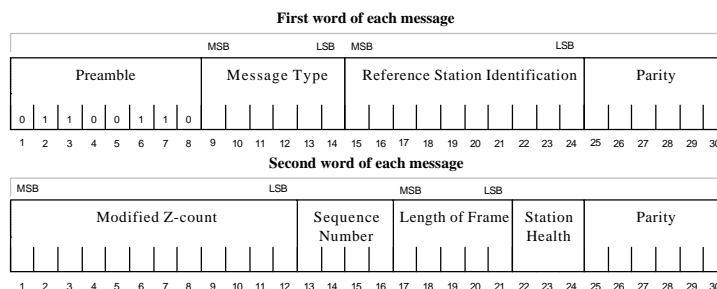
Figure 2.3 – RTCM Header.
