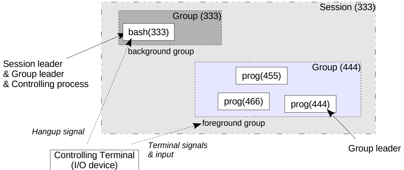
Fig. Inter-relationships of processes, groups, sessions and input/output terminal.
