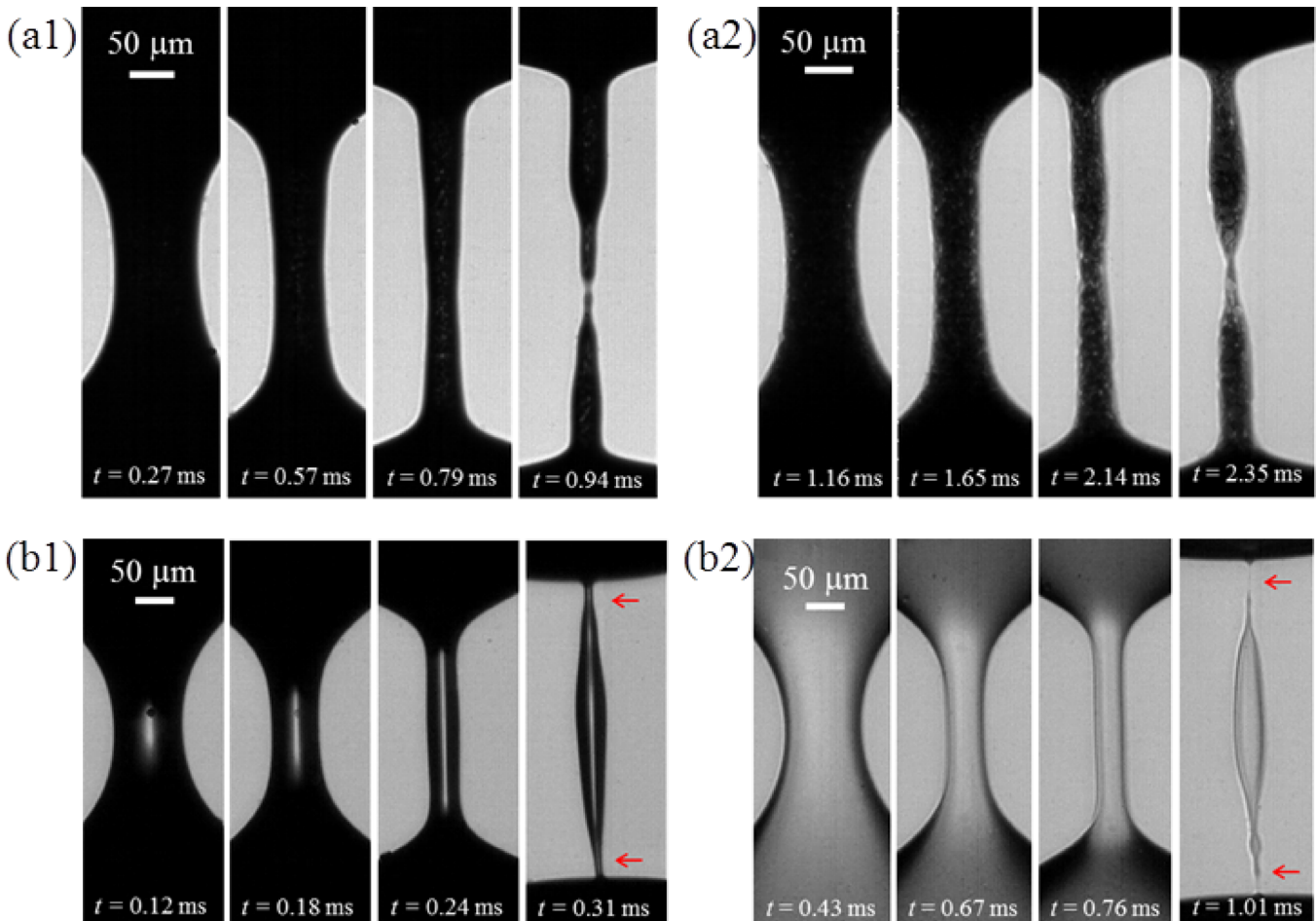
FIG. 4. Sequence of images showing the evolution of a filament of whole human blood (a1) and (a2) and human plasma (b1) and (b2) at four instants of time. Images (a1) and (b1) correspond to measurements in air, whereas images (a2) and (b2) correspond to measurements in the silicone oil. All blood and plasma samples shown were collected from donor D3.
