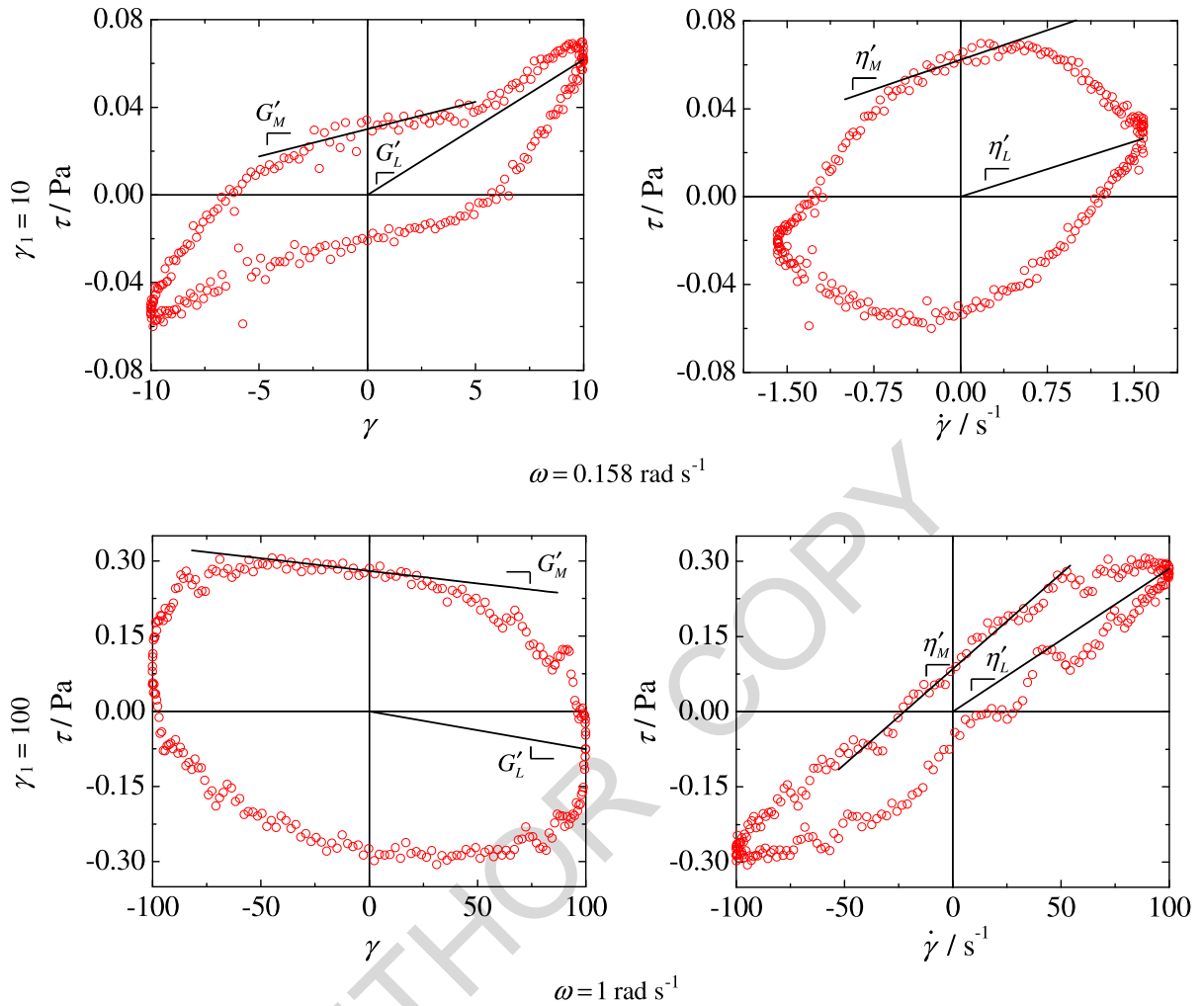
Fig. 4. Lissajous–Bowditch plots for two different strain amplitudes and angular velocities. The slopes of the lines represent the variables G'_M , G'_L , \eta'_M and \eta'_L . Blood samples from donor A. (Colors are visible in the online version of the article; http://dx.doi.org/10.3233/BIR-130643 .)
