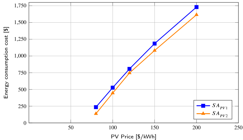
Fig. 15. Sensitivity analyzing on PV cost (β = 0.9).
