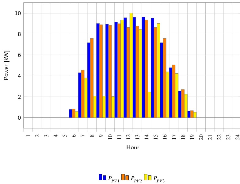
Fig. 14. Power generated by the PV in summer (β = 0.9).
