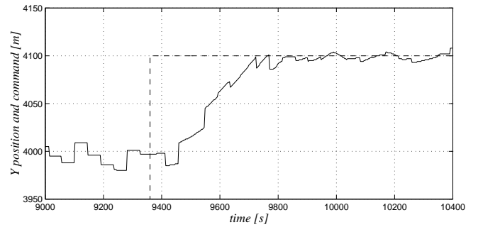
Figure 8: Commanded and measured Y position.
