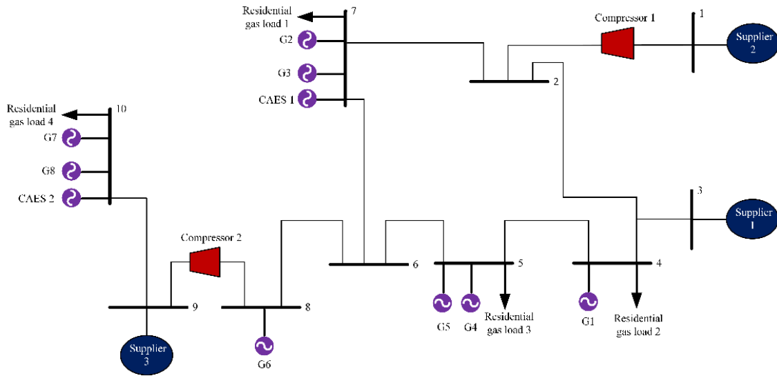
Fig. 15. Ten-node natural gas system
