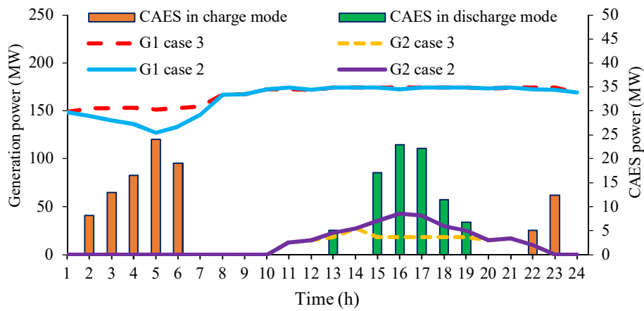
Fig. 10. Effect of CAES unit on hourly power generation dispatch of G1 and G2
