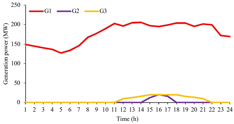
Fig. 4. Hourly power generation dispatch for case 1
