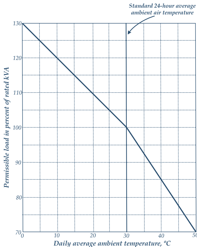
Figure 5. Permissible kVA loading by varying \theta_a for natural cooled transformers.
