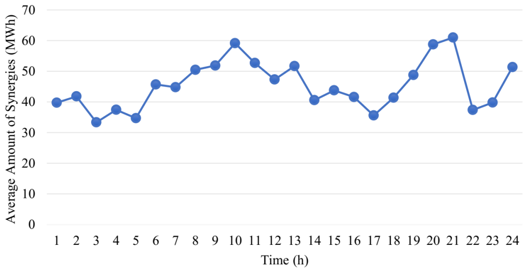
Figure 11 Average amount of SR synergy between the Iberian TSOs.
