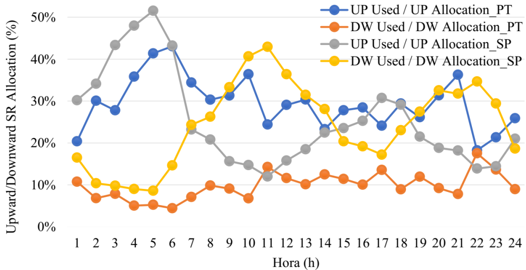
Figure 2 Upward and Downward SR allocation between the Iberian TSOs.
