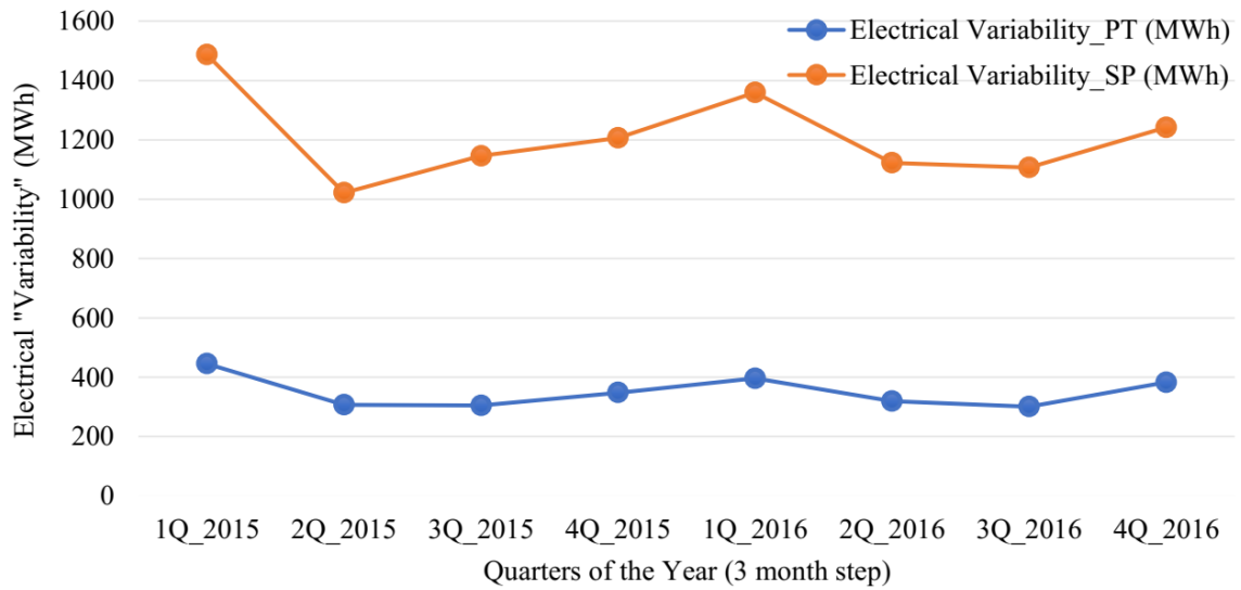
Figure 7 “Electrical variability” comparison behavior between the Iberian TSOs.
