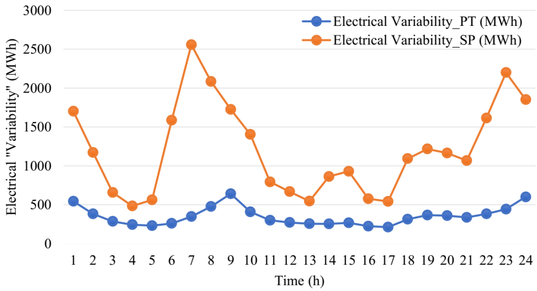
Figure 3 “Electrical variability” between the Iberian TSOs.
