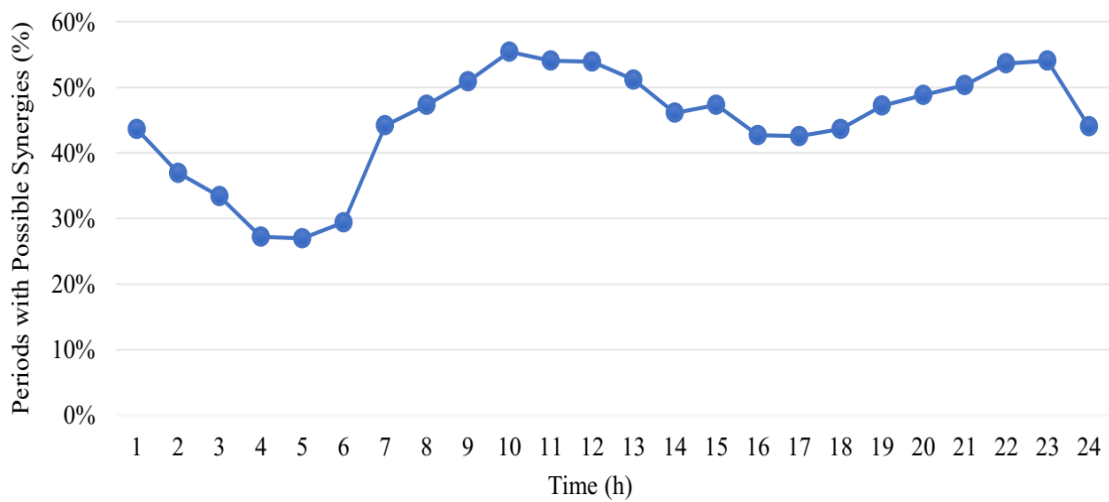
Figure 10 Periods of possible SR synergy between the Iberian TSOs.
