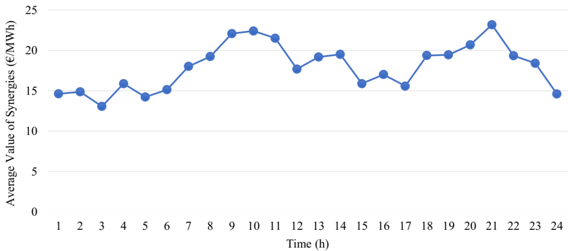
Figure 12 Average price value of synergy occurred between the Iberian TSOs.
