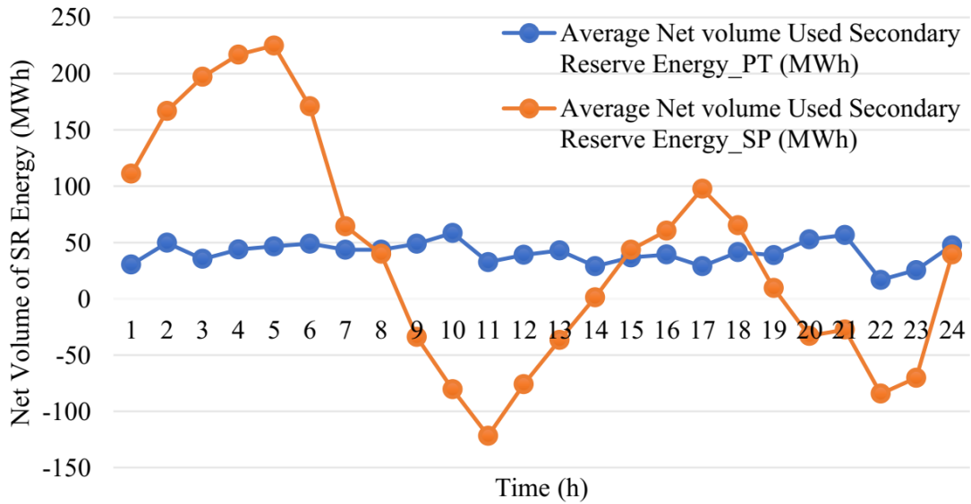
Figure 1 Average net volume used on the SR with Iberian TSOs.
