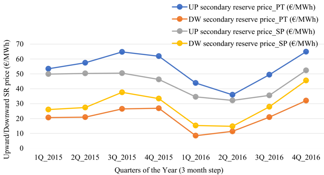
Figure 6 Upward and downward SR prices practiced by the Iberian TSOs.
