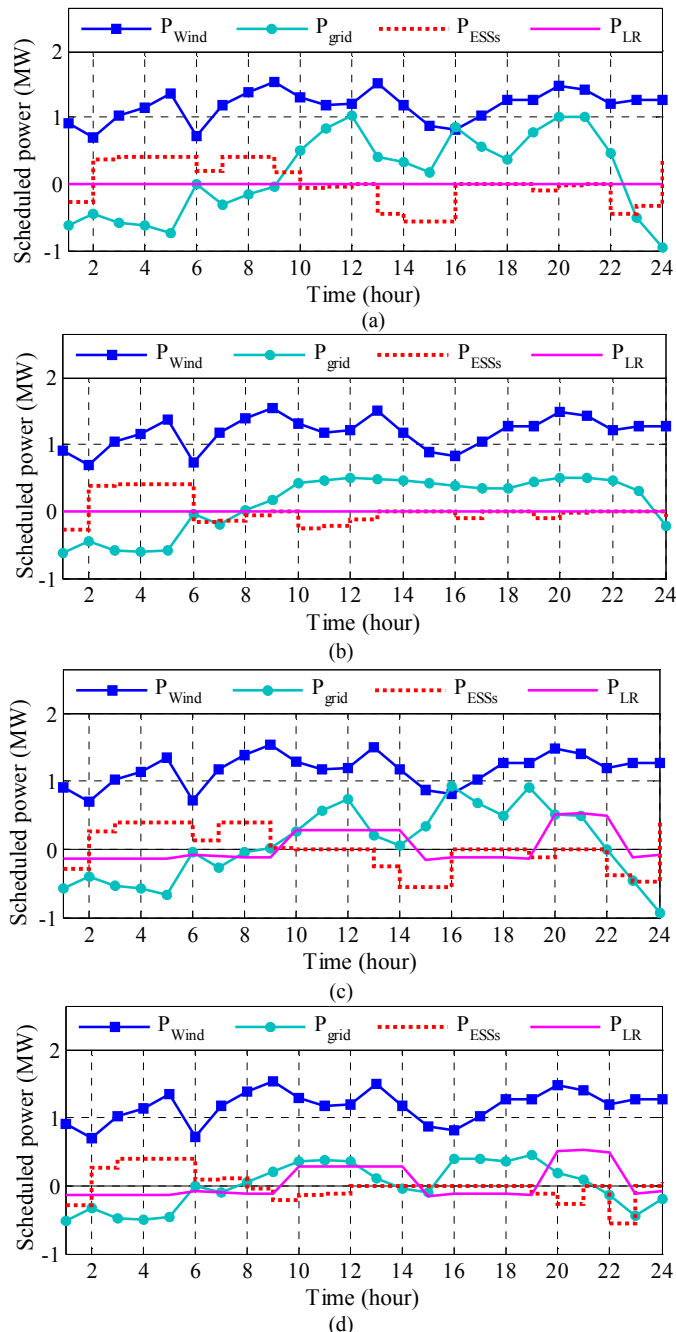
Fig. 8. Hourly power of the VPP's elements, (a) without DR in the risk-neutral decision (b) without DR in the risk-averse decision, (c) with DR in the risk-neutral decision, and (d) with DR in the risk-averse decision.
