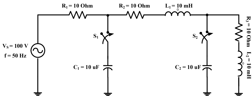
Fig.3 Single line diagram of single phase simple test system [35]
