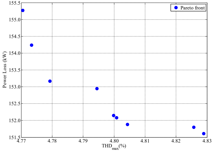
Fig. 13 Optimal Pareto Front for the 85-Bus Test System
