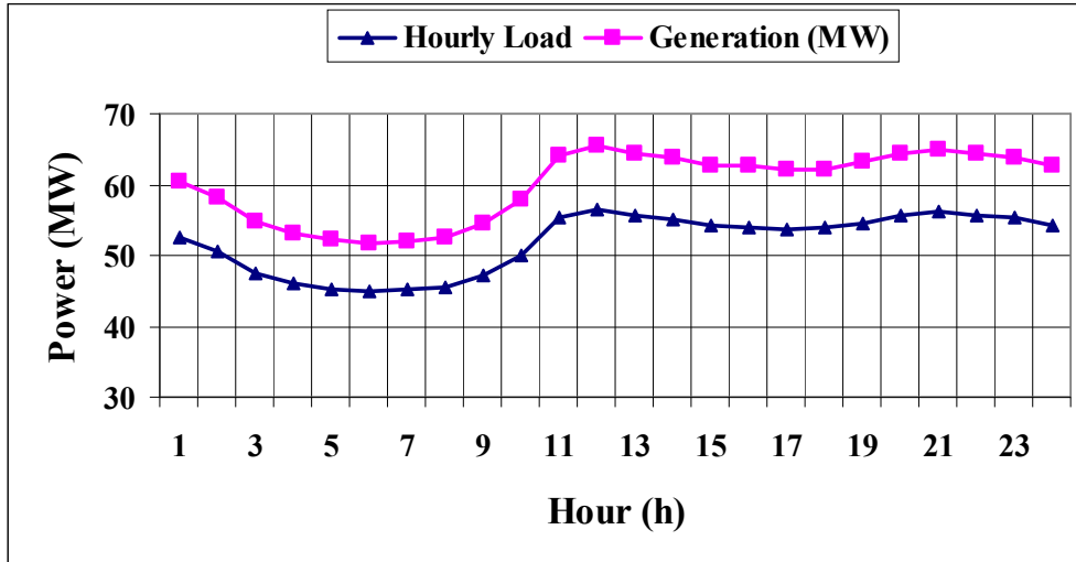
Fig. 12 Demand and generation power trends for daily peak load
