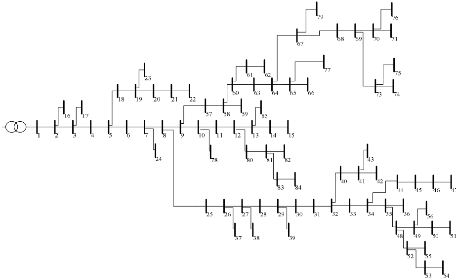
Fig. 11 Single line diagram of 85-bus test system [41]
