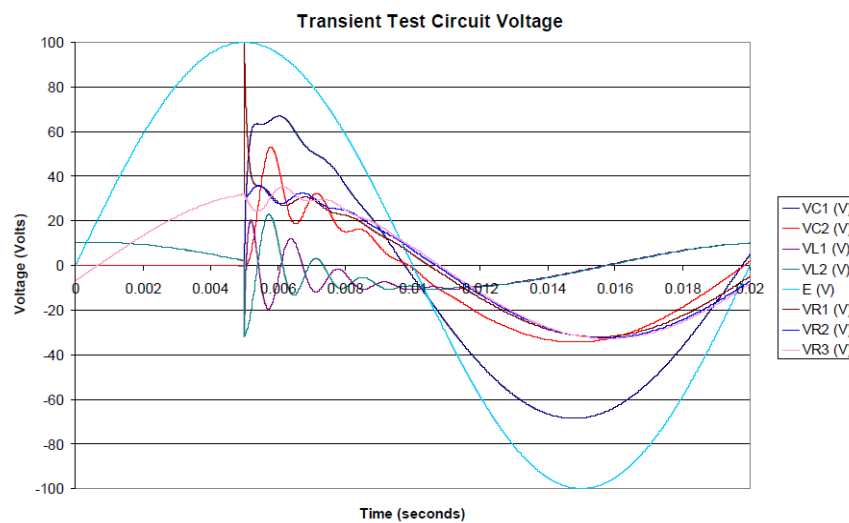
Fig. 4 The worst case capacitor switching at peak voltage (ATP) [35]
