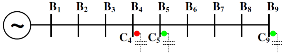
Fig 1. Classical mapping procedure to address the capacitor placement problem
