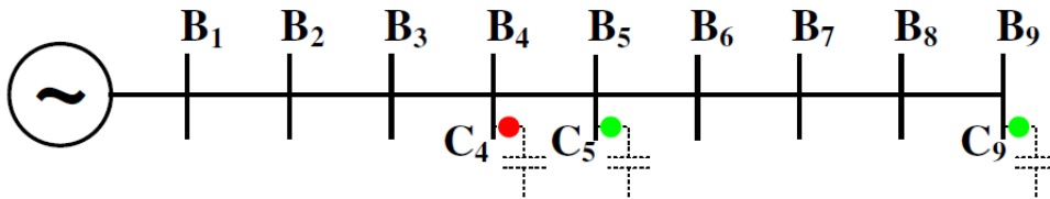
Fig2. Modified capacitor placement with local search technique
