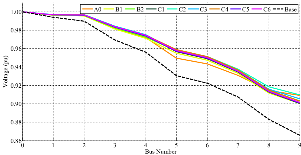
Fig. 8 Voltage profile of 9-bus test system
