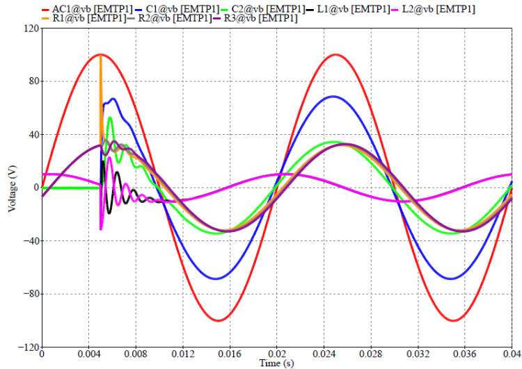
Fig. 5 The worst case capacitor switching at peak voltage (EMTP-RV)
