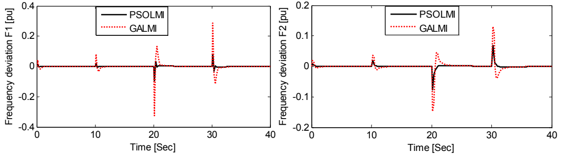
(a) Frequency deviation in area-1 (b) Frequency deviation in area-2
