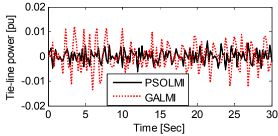
(c) Tie-line power deviation
