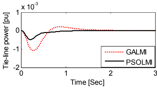
(c) Tie-line power deviation
