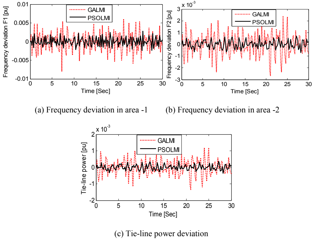
Fig. 13. Response for case study-2 with random wind power variation
