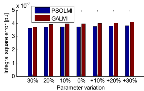
Fig. 16. Computed ISE for change in all system parameters
