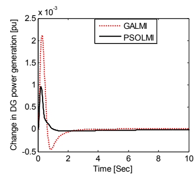
(f) Change in total DG power generation
