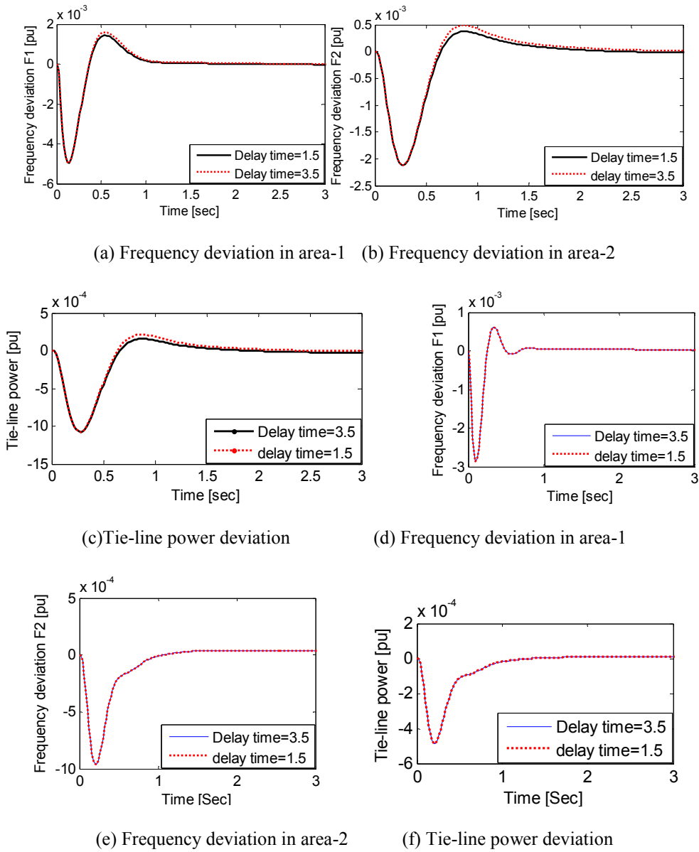
Fig. 15. Response for case study-2 with time delays
