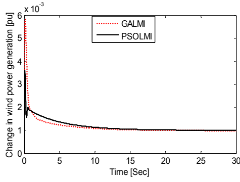
(a) Change in wind power generation
