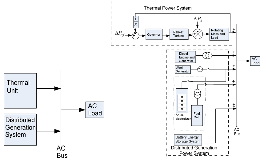
(a) Block diagram
