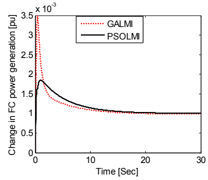
(c) Change in FC power generation
