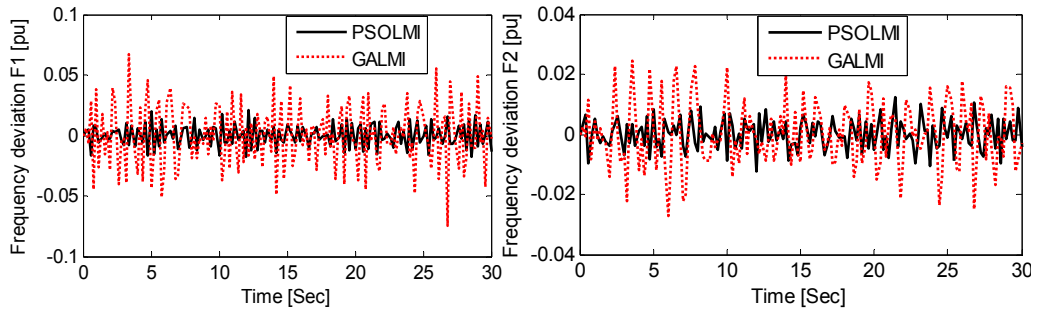
(a) Frequency deviation in area-1 (b) Frequency deviation in area-2
