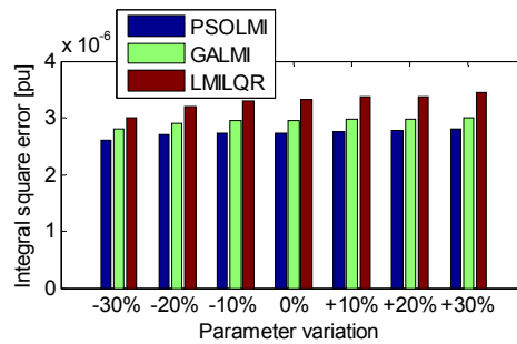
Fig. 9. Computed ISE for uncertainties in all system parameters
