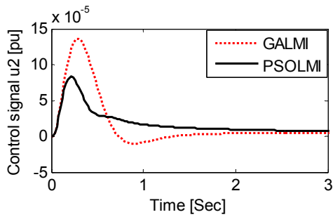
(g) Control signal u_2
