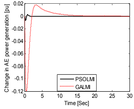
(b) Change in AE power generation
