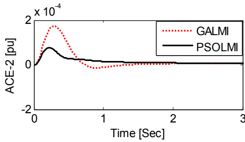
(e) ACE in area-2
