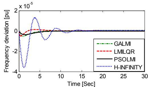
Fig. 4. Response with step load change
