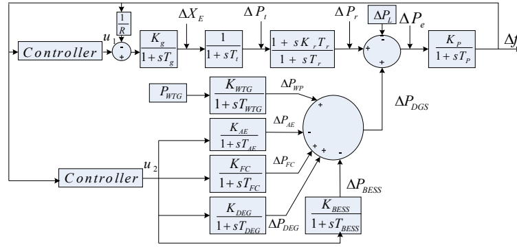
(b) Transfer function model
