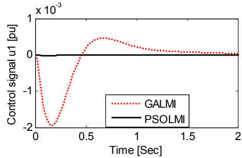
(f) Control signal u_1
