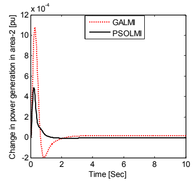
(h) Change in power generation in area-2
