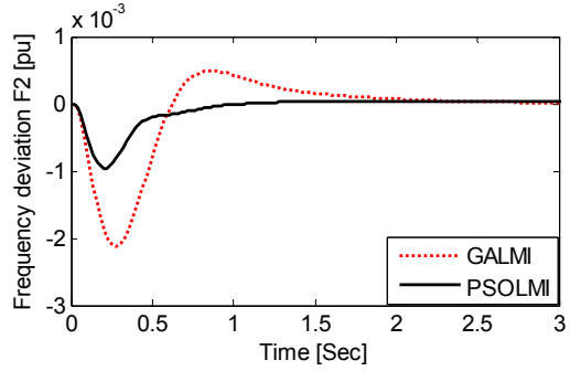
(b) Frequency deviation in area-2
