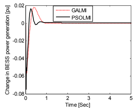
(e) Change in BESS power generation
