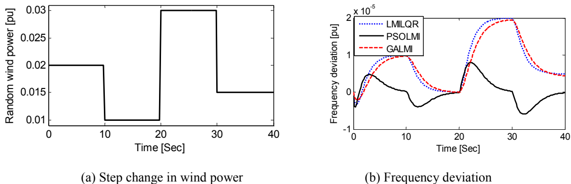
Fig. 7. Response for case study-1 with step change in wind power
