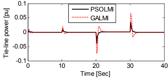
(c) Tie-line power deviation
