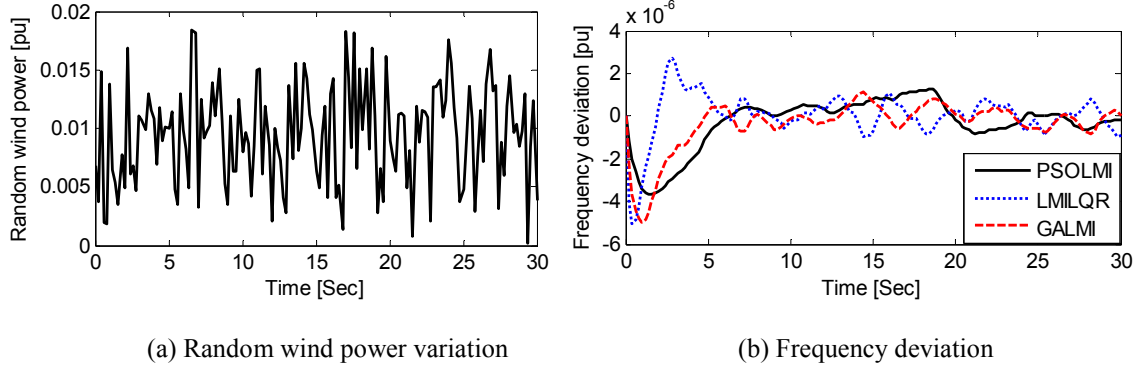
Fig. 8. Response with random wind power variation
