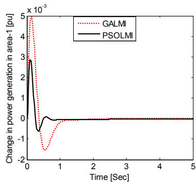
(g) Change in power generation in area-1
