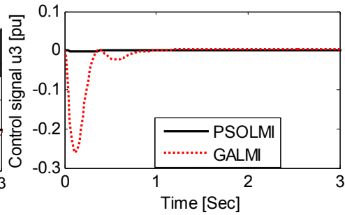
(h) Control signal u_3
