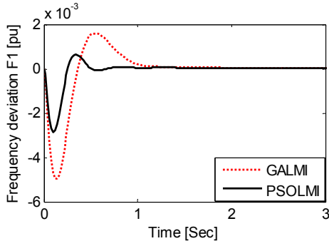
(a) Frequency deviation in area-1
