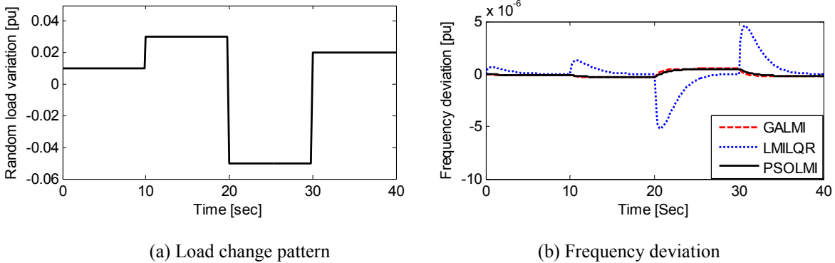
Fig. 5. Response with random step load change
