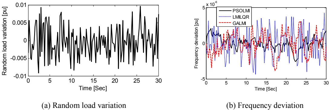
Fig. 6. Response with random load variation
