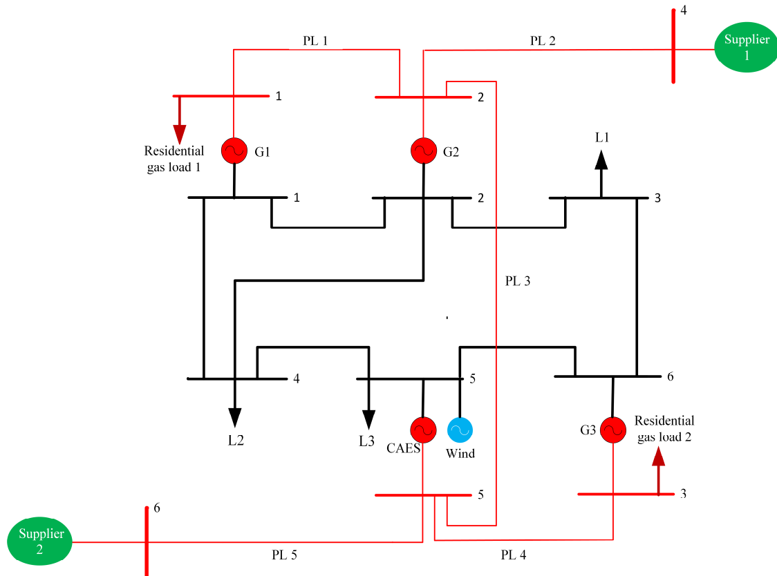
Fig. 3. Illustration of 6-bus electrical and 6-node natural gas systems with wind and CAES unit
