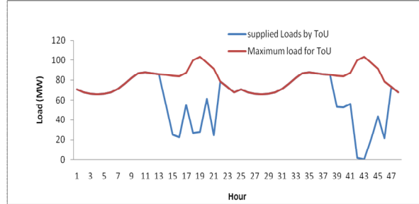
Fig.2 Maximum load for joining ToU and the amount of supplied loads within ToU program
