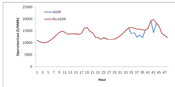
Fig.3 Hourly operation cost for case 3 and 4
