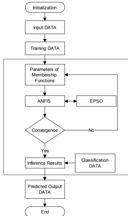
Fig. 1. Flowchart of the novel EPA approach.
