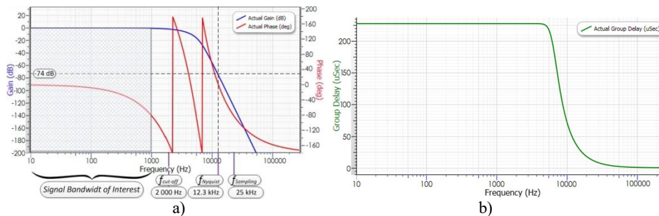
Fig.4. 10th order Bessel filter frequency response: a) Magnitude and phase; b) Group delay.
