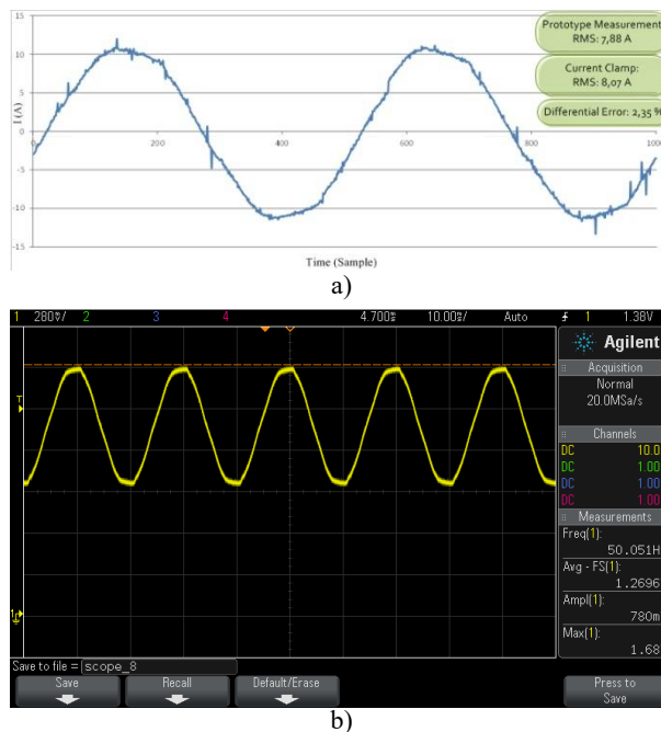
Fig.7. Full power operating electric space heater: a) Prototype acquired current profile; b) ACS712 output.
