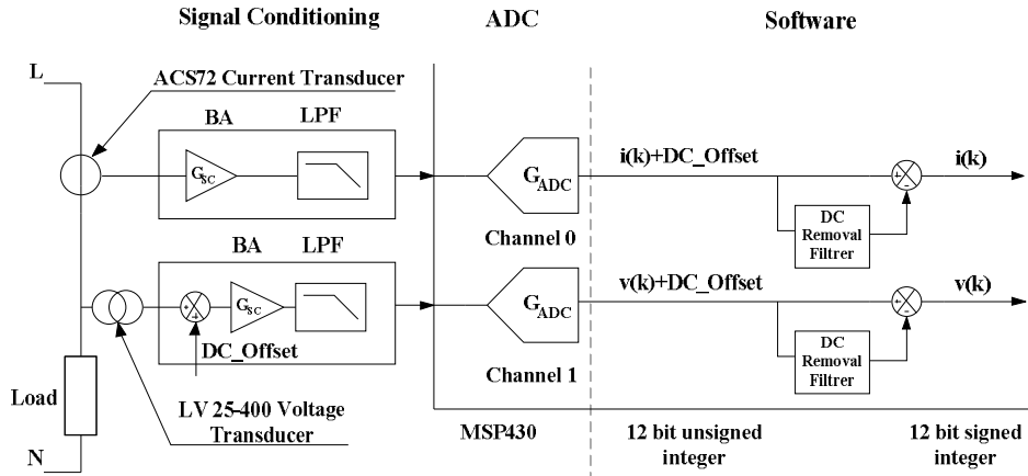
Fig.3. Sensing, acquisition and post-filtering block diagram.
