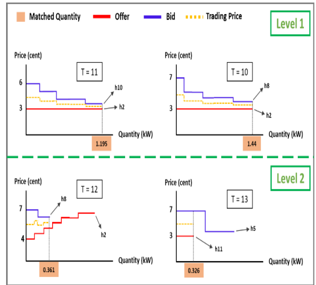
FIGURE 9. Examples of matching of prosumers' offers with consumers' bids considering the proposed model.
