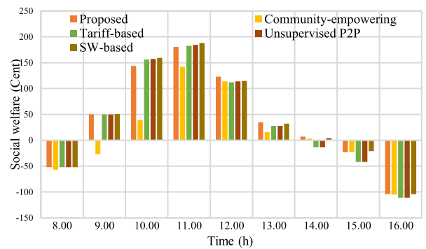
FIGURE 10. Hourly SW index of the households.
